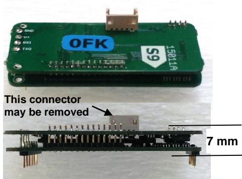
15011 OEM Modem Assembly (S9 Footprint)
